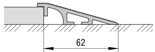
ramp rail RS 14
