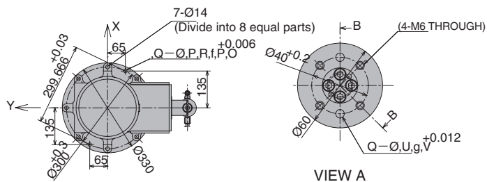
INSTALLATION DIMENSIONS
