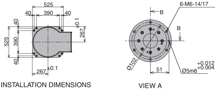
INSTALLATION DIMENSIONS
