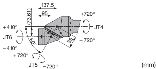
INSTALLATION DIMENSIONS
