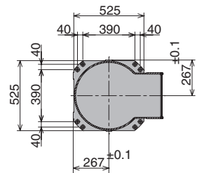
INSTALLATION DIMENSIONS
